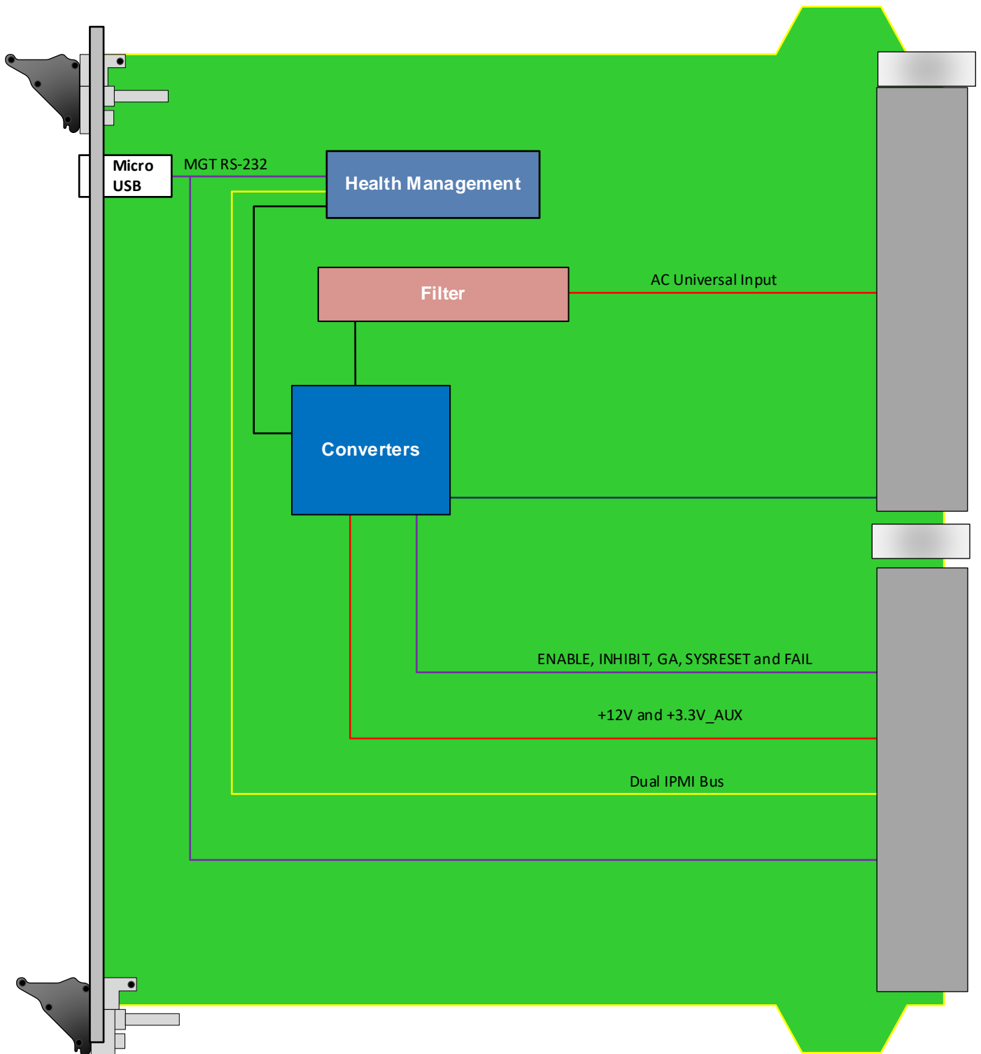
Figure 2: VPX028 Functional Block Diagram
