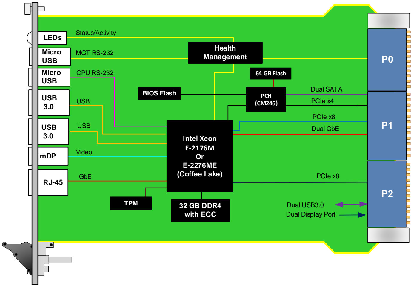
Figure 2: VPX760 Functional Block Diagram
