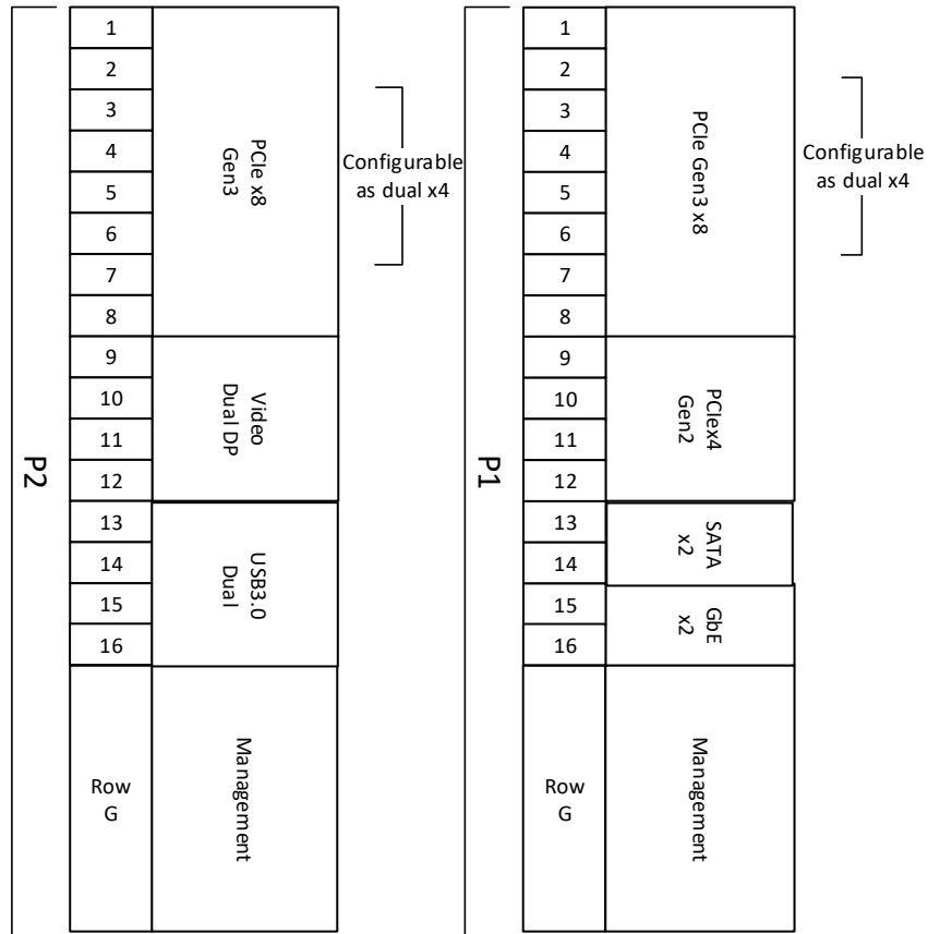
Figure 4: VPX760 Pinout Block Diagram
