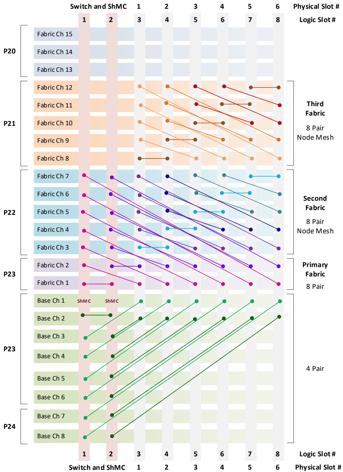
Figure 3: VT831 Backplane Flush Mesh with a Replicated Mesh on Node slots
