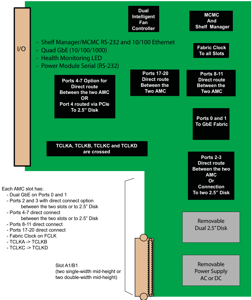
FIGURE 1. VT855 Functional Block Diagram
