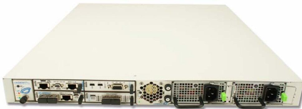
VT857 rear view with AC input supply
