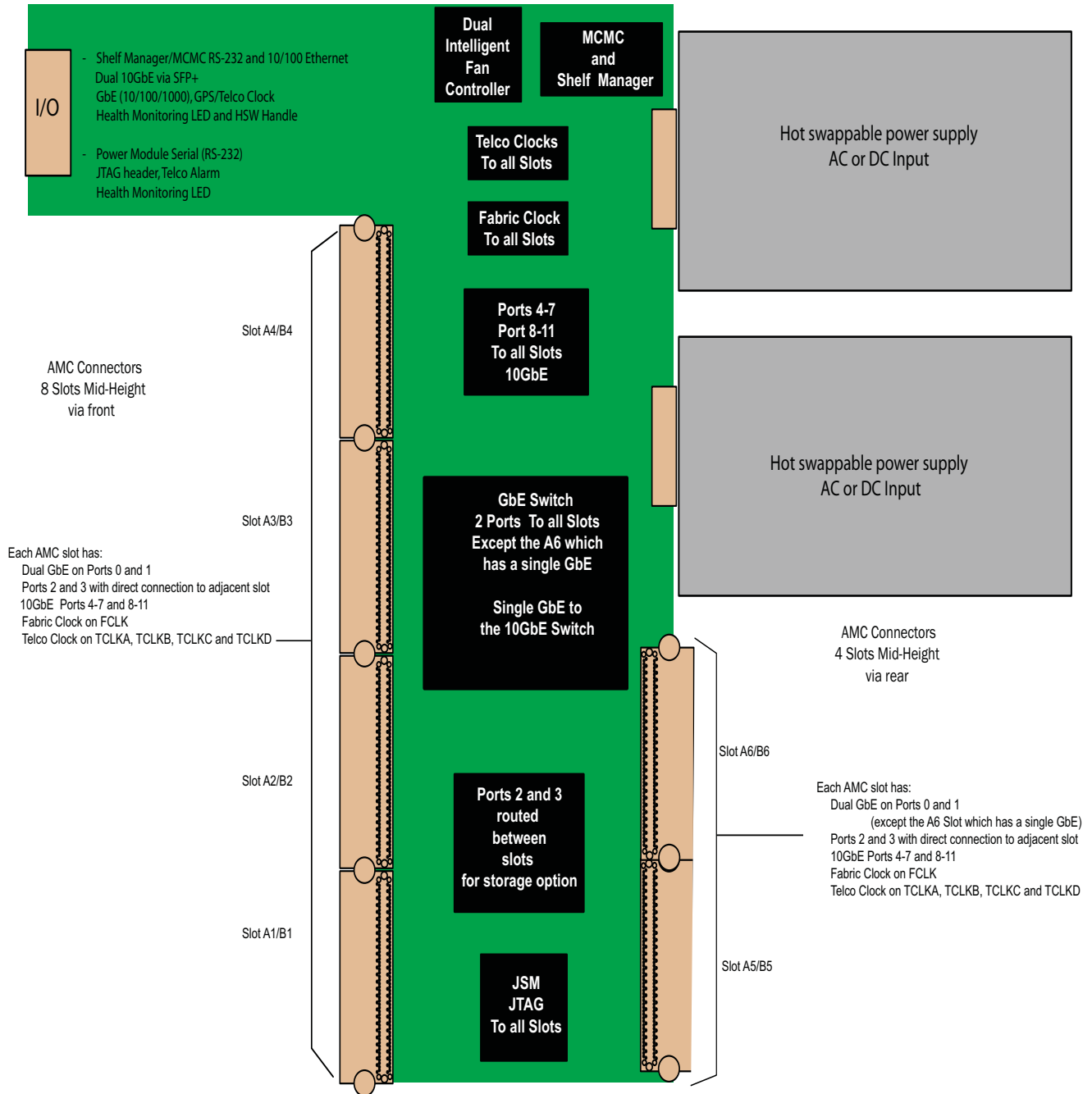
FIGURE 1. VT857 Functional Block Diagram
