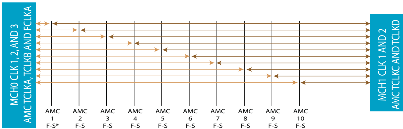
FIGURE 6. VT865 AMC 2.0 Enhanced Clock Redundancy Topology
