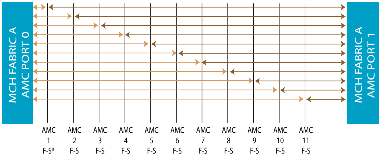
FIGURE 2. VT893 Topology for AMC Ports 0 and 1
