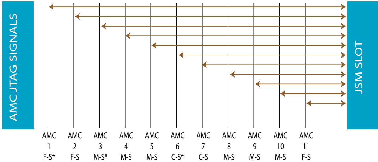
FIGURE 5. VT893 Topology for JSM
