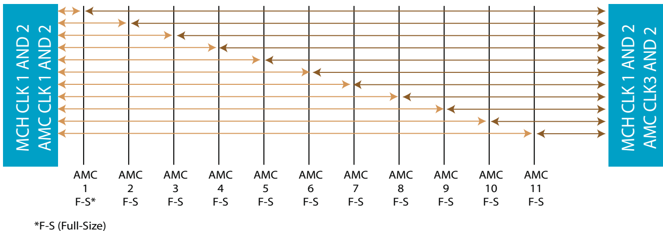
FIGURE 7. VT893 redundant clock Topology
