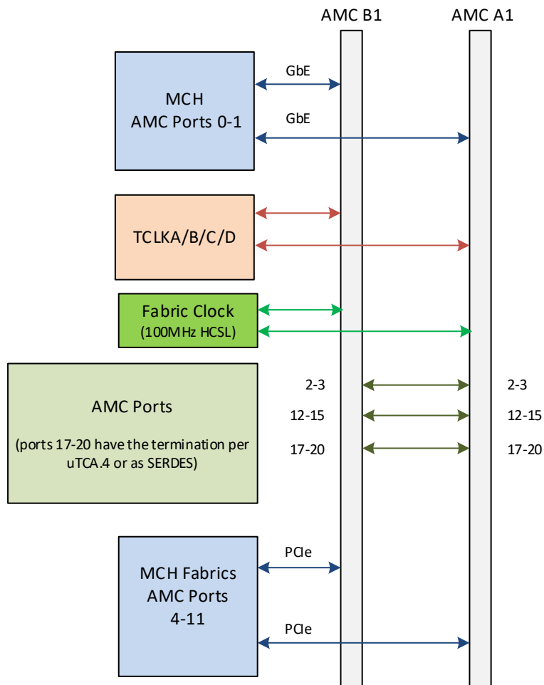
Figure 4: VT806 Backplane Connections
