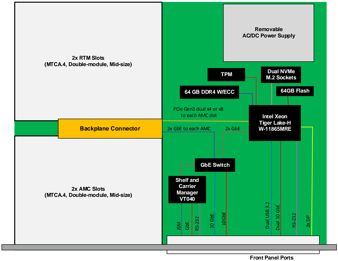
Figure 3: VT806 Block Diagram
