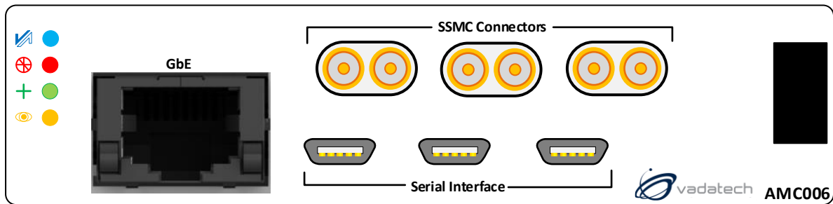
Figure 3: AMC006 Front Panel
