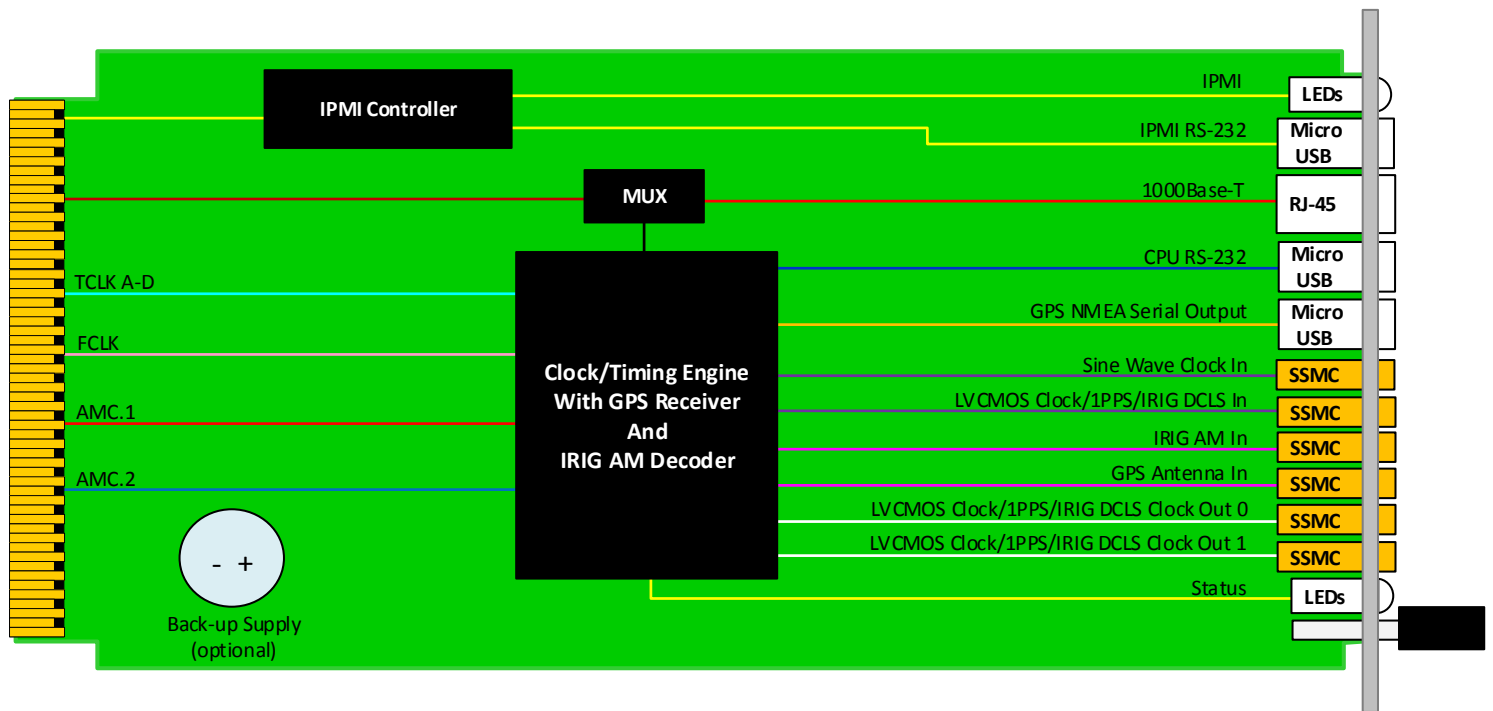
Figure 2: AMC006 Functional Block Diagram
