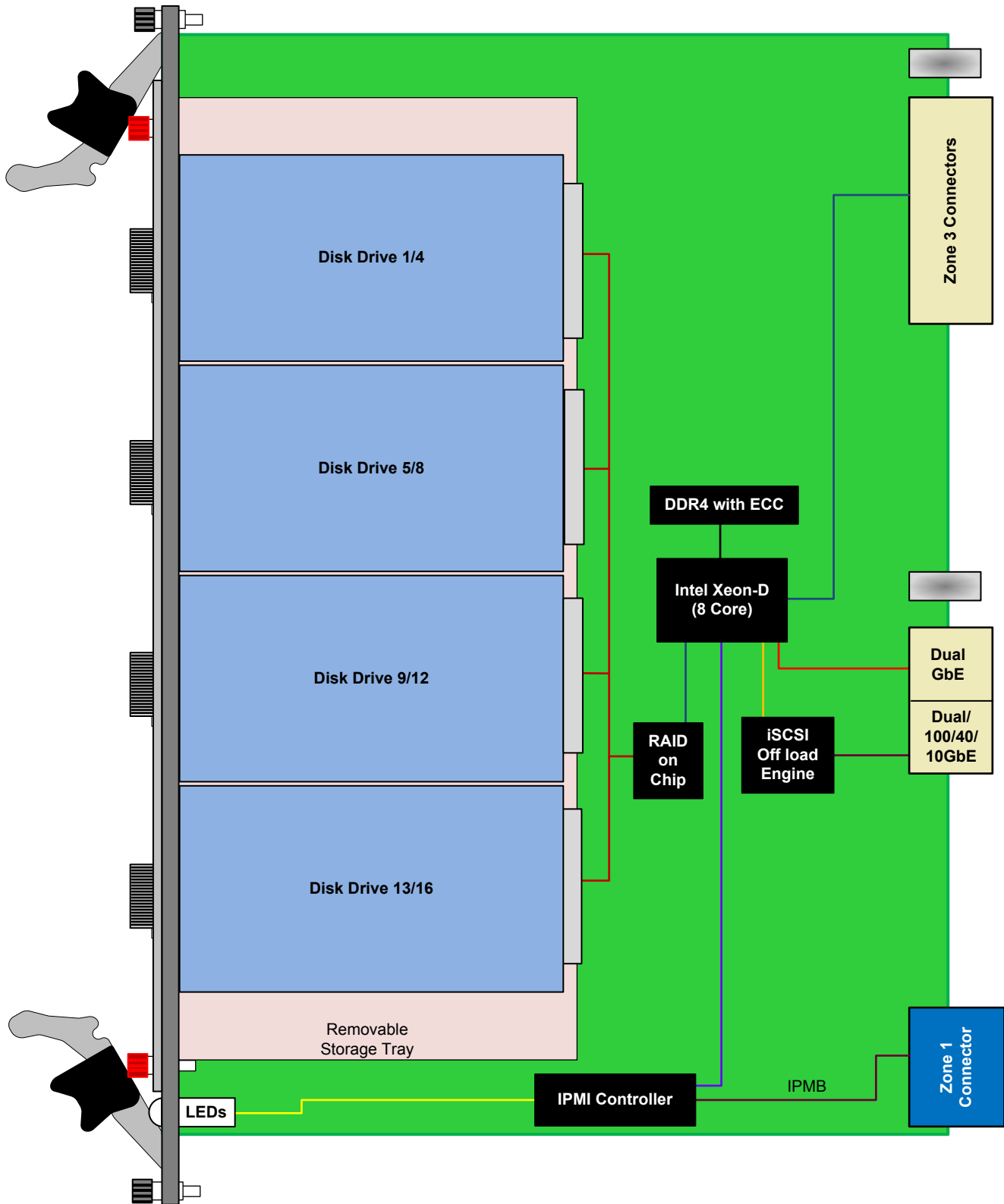
Figure 4: ATC600 Functional Block Diagram
