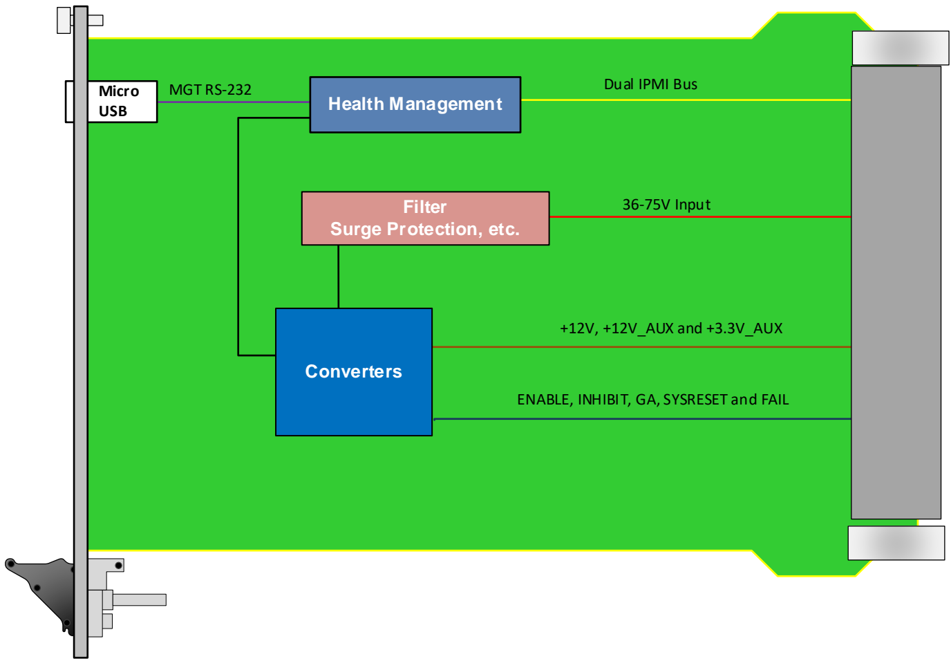
Figure 2: VPX029 Functional Block Diagram
