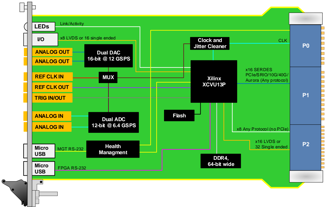
Figure 2: VPX589 Functional Block Diagram
