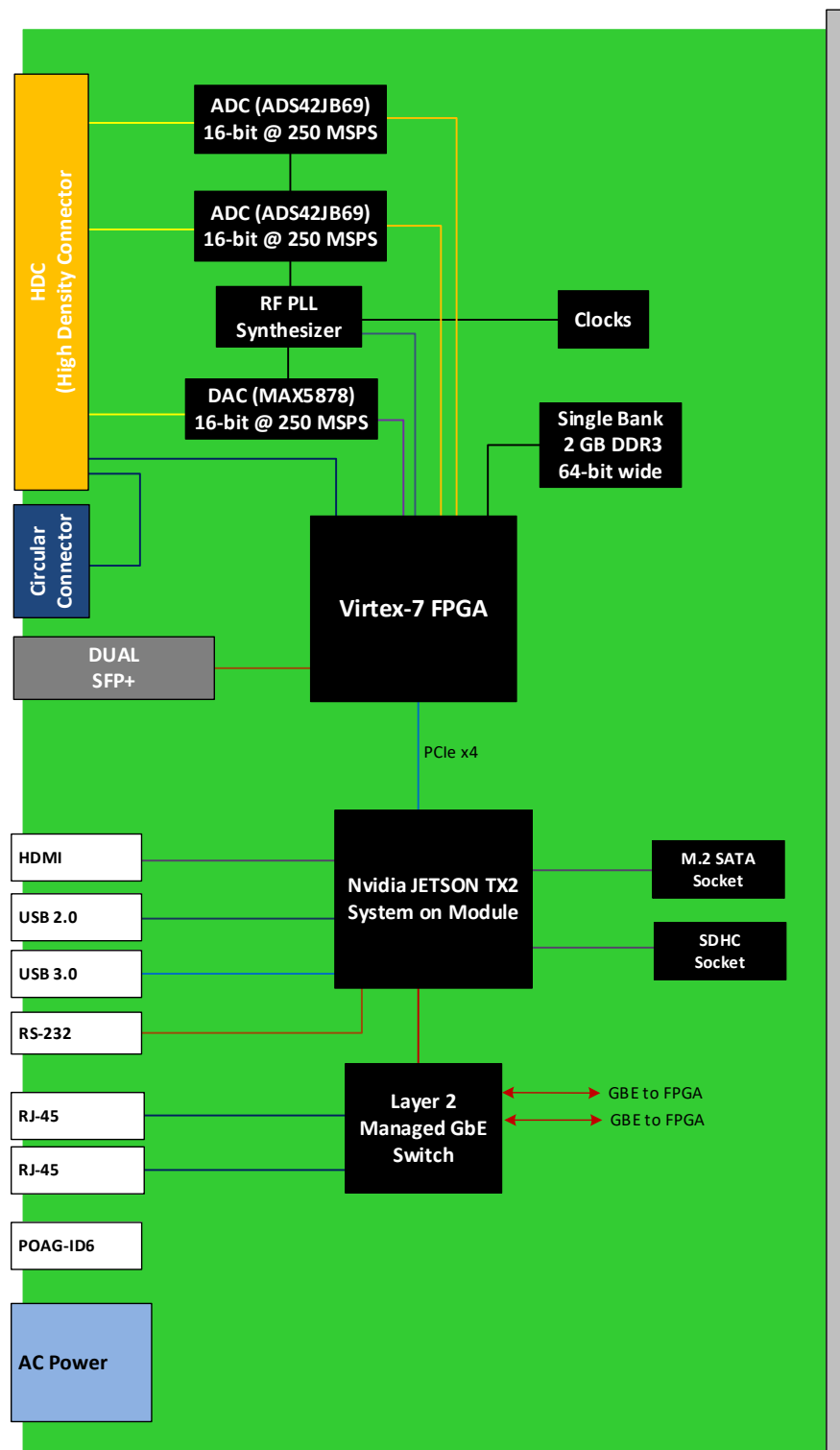
Figure 3: VT983 Functional Block Diagram
