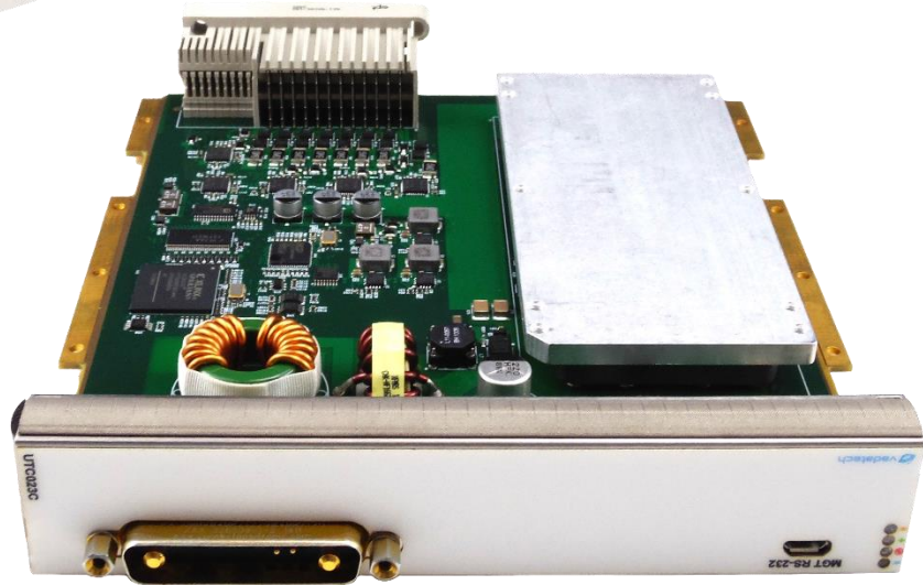
Figure 2: UTC023 without Cover
