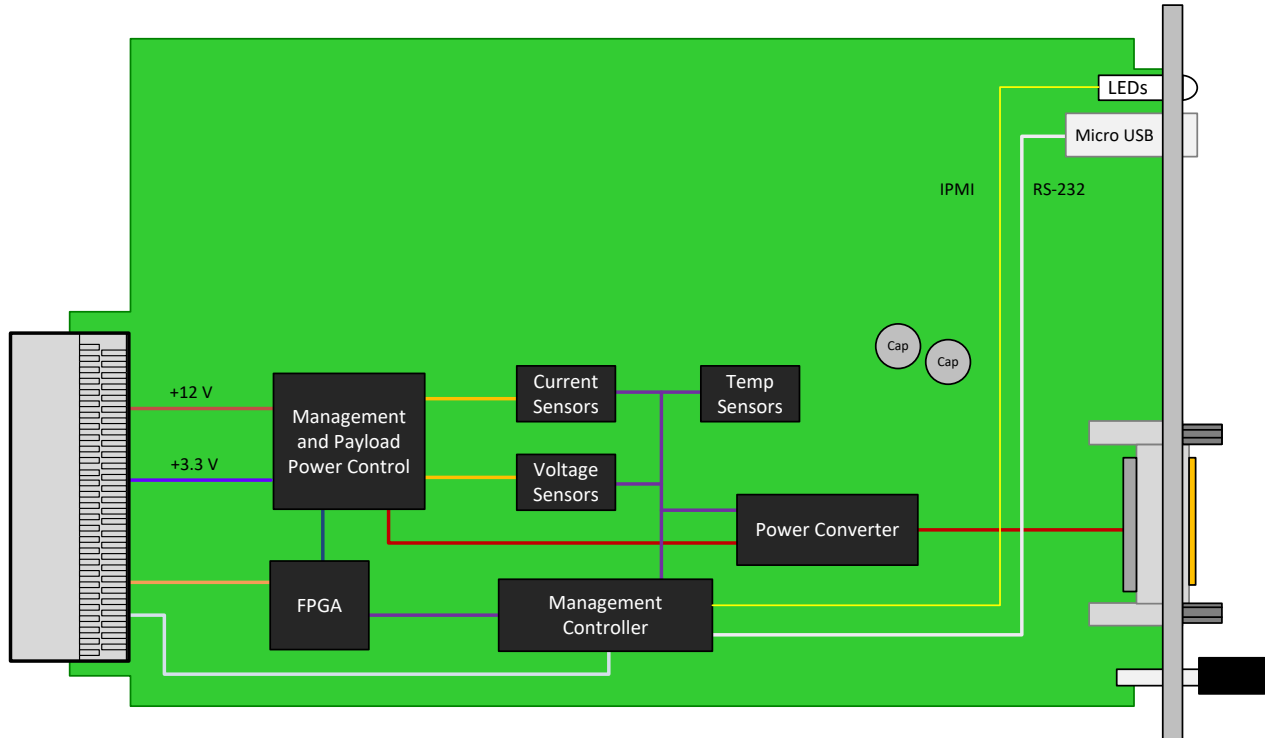
Figure 4: Block Diagram – Air Cooled Version
