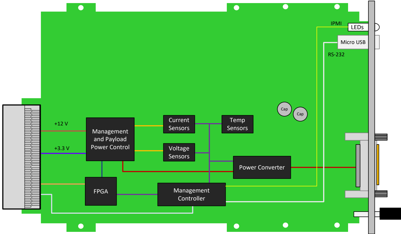
Figure 6: Block Diagram - Conduction Cooled Version
