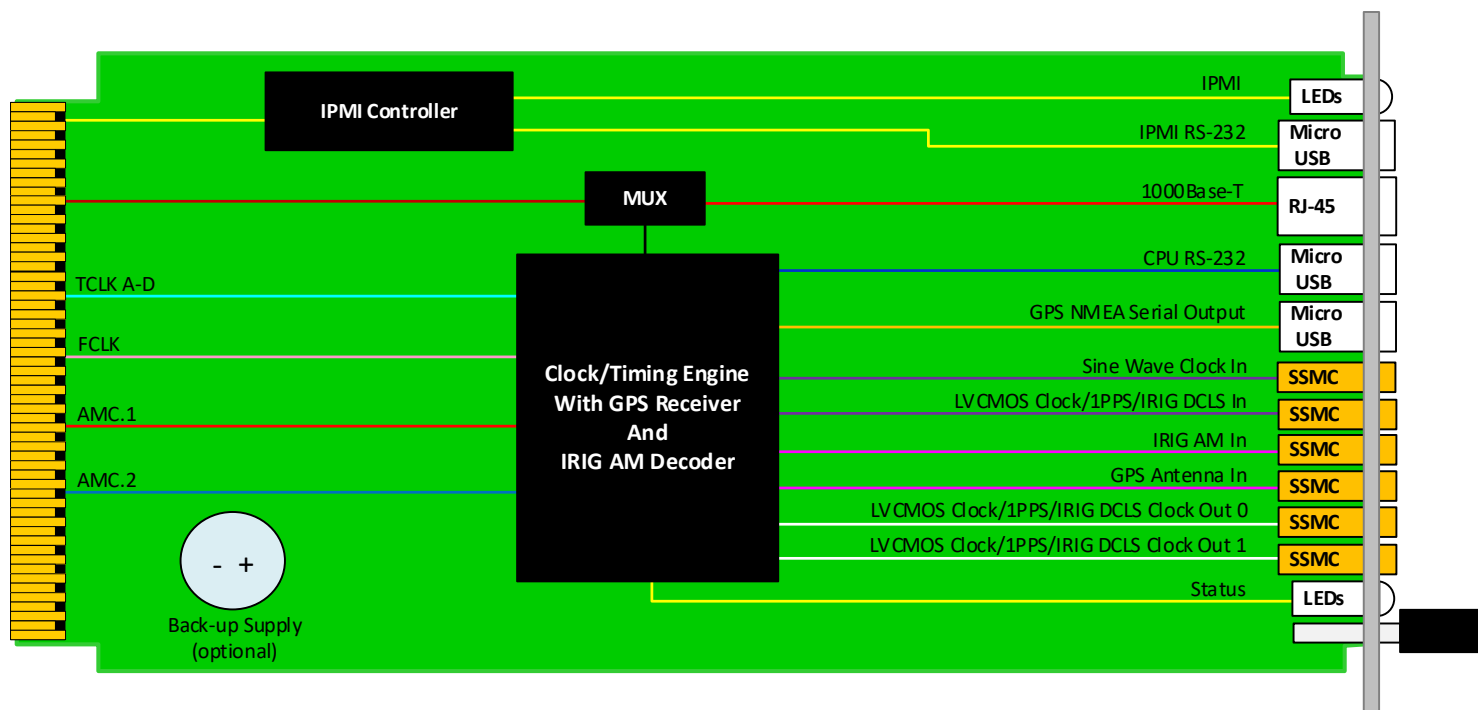
Figure 2: AMC006 Functional Block Diagram
