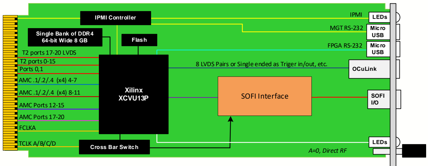
Figure 7: AMC547 Functional Block Diagram
