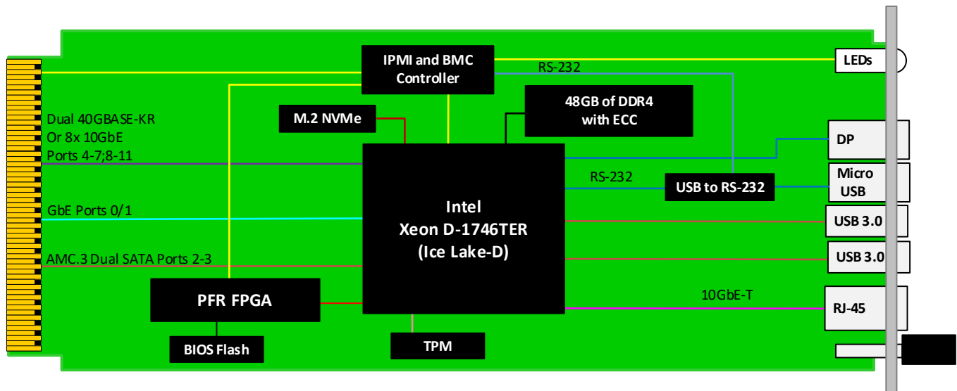
Figure 3: AMC770 Functional Block Diagram
