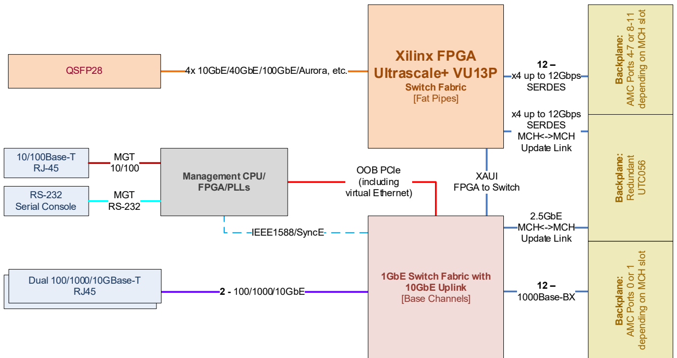
Figure 12: UTC055 Connectivity and Fabric option FPGA
