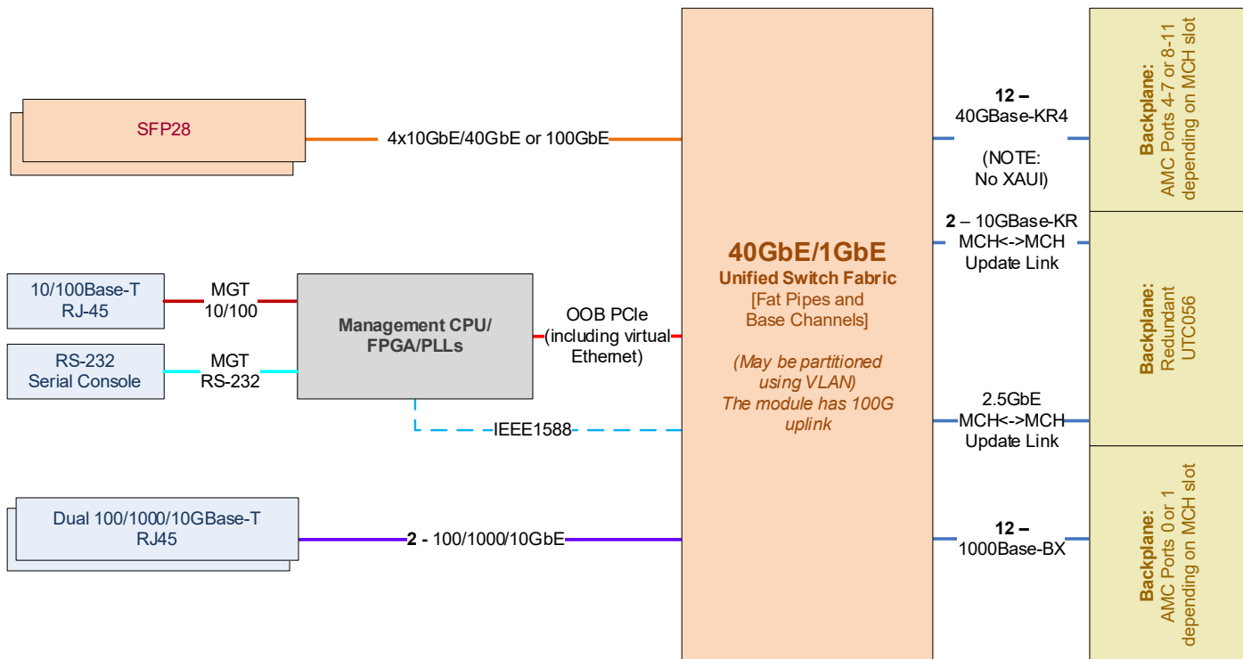
Figure 8: UTC055 Connectivity and Fabric Option 40GbE with dual SFP28
