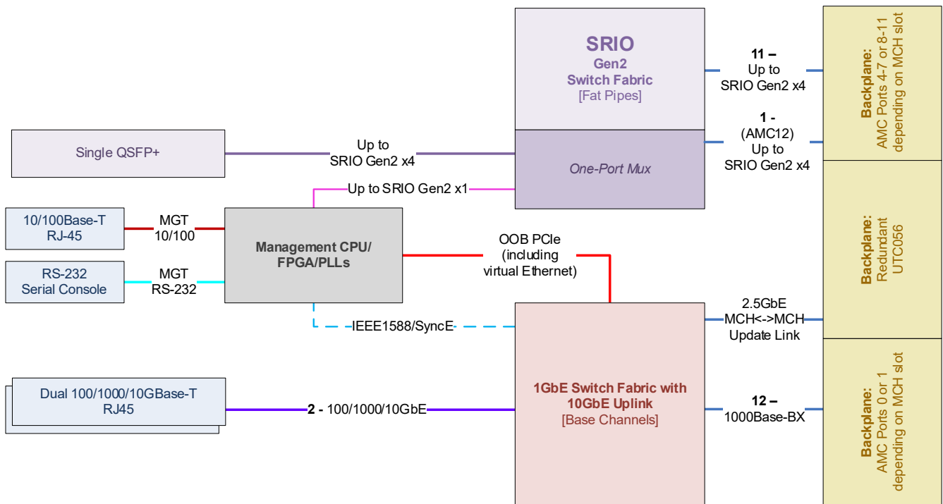
Figure 11: UTC055 Connectivity and Fabric option PCIe
