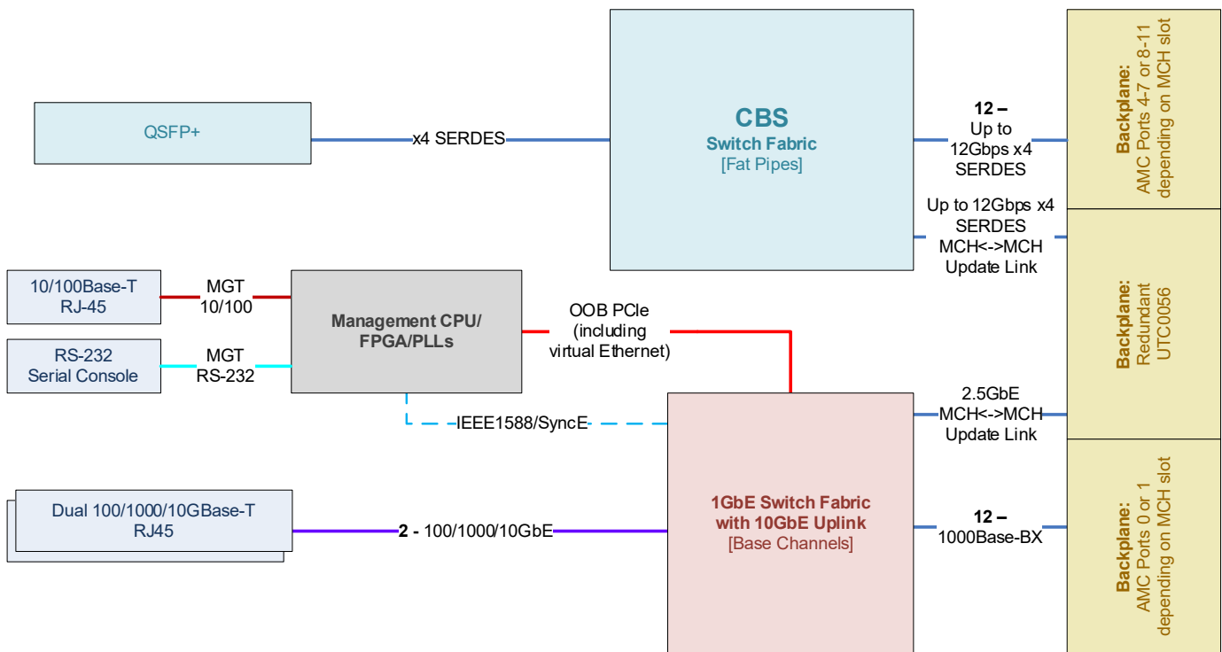
Figure 13: UTC055 Connectivity and Fabric Options Cross Bar Switch (CBS)
