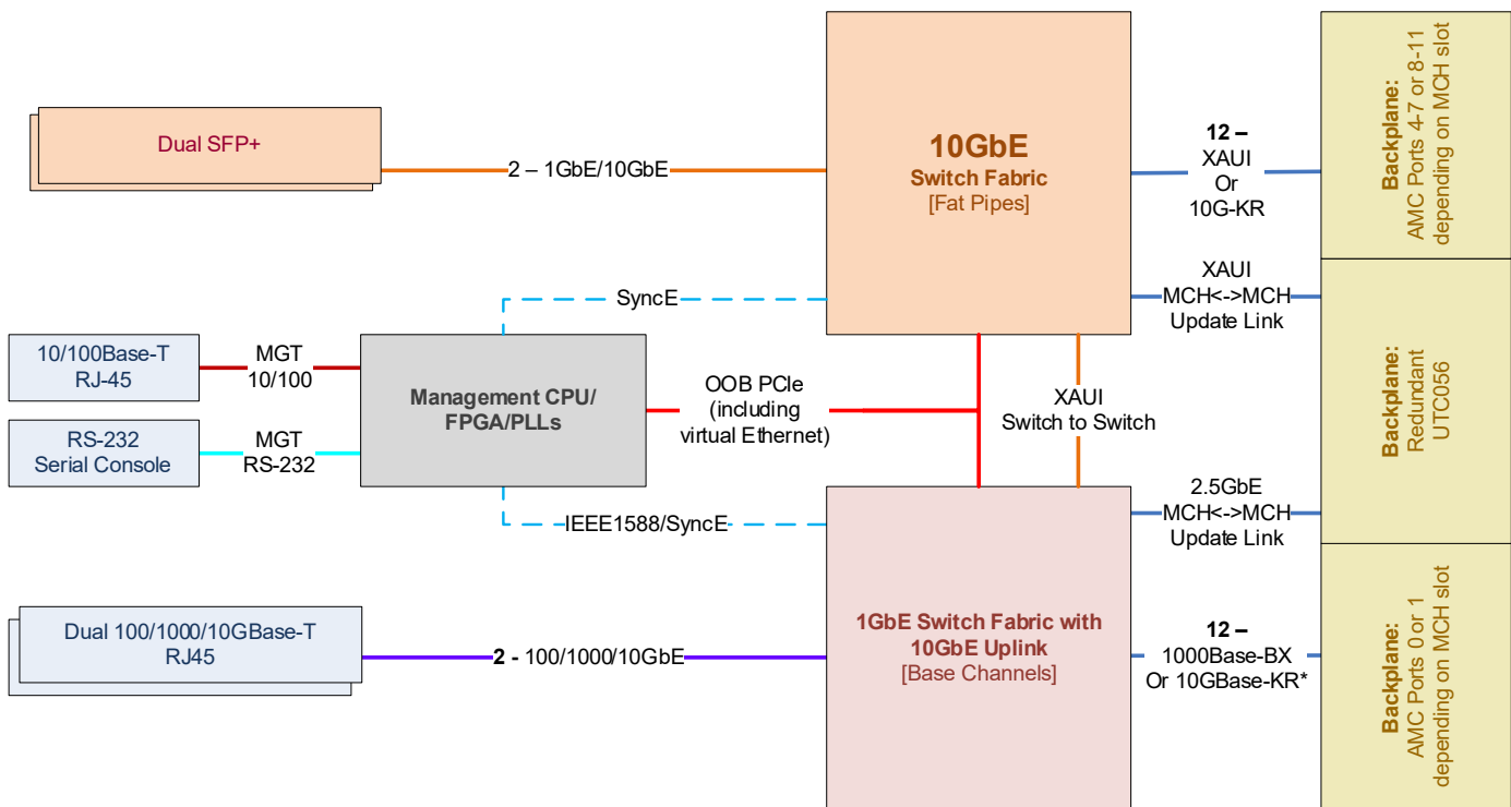
Figure 9: UTC055 Connectivity and Fabric Option 10GbE with Dual SFP+
