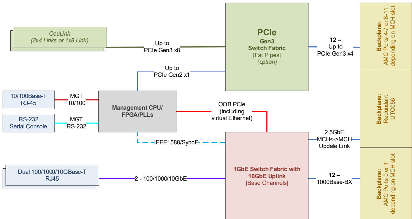
Figure 10: UTC055 Connectivity and Fabric option PCIe
