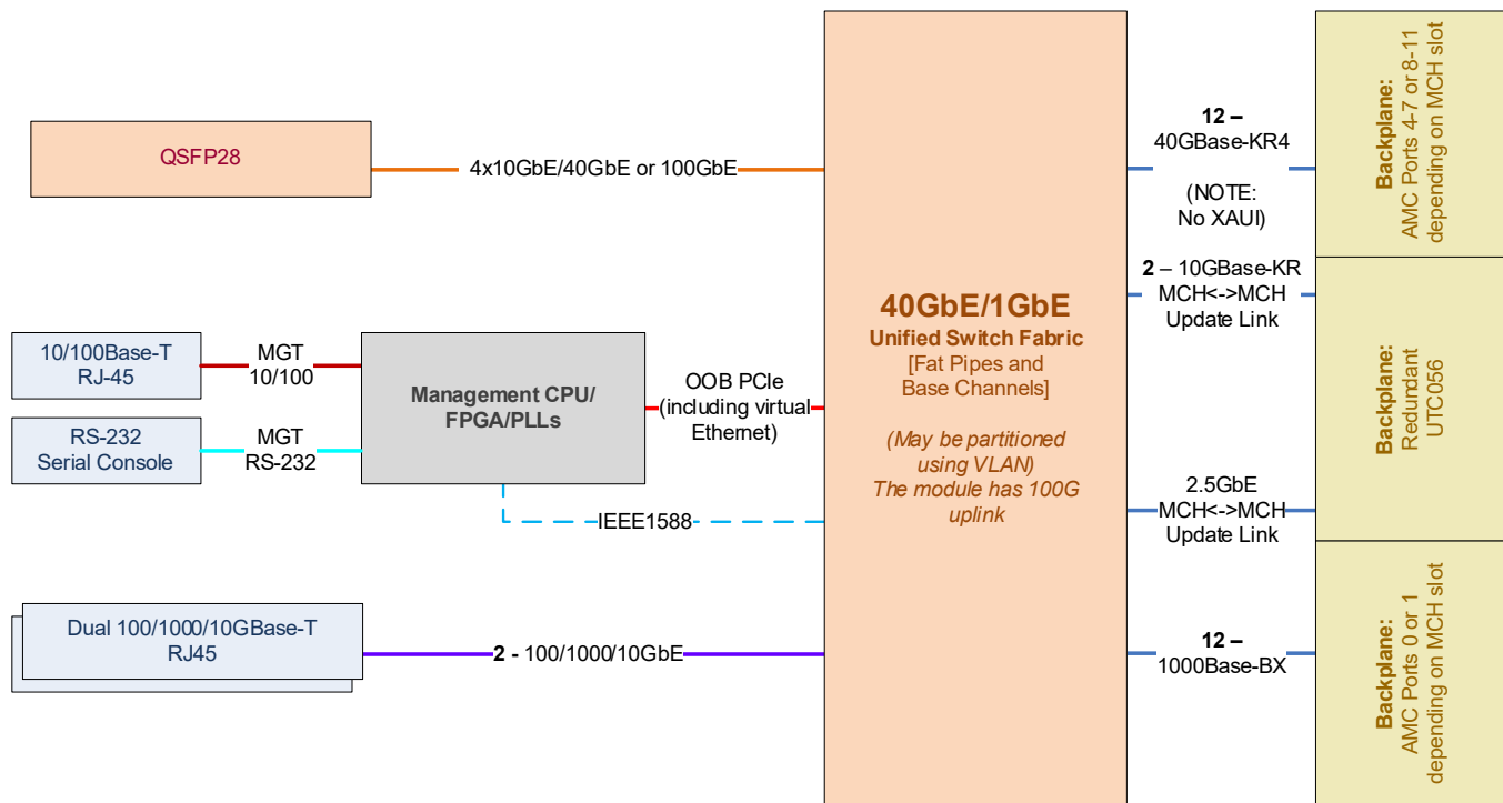
Figure 7: UTC055 Connectivity and Fabric Option 40GbE with QSFP28
