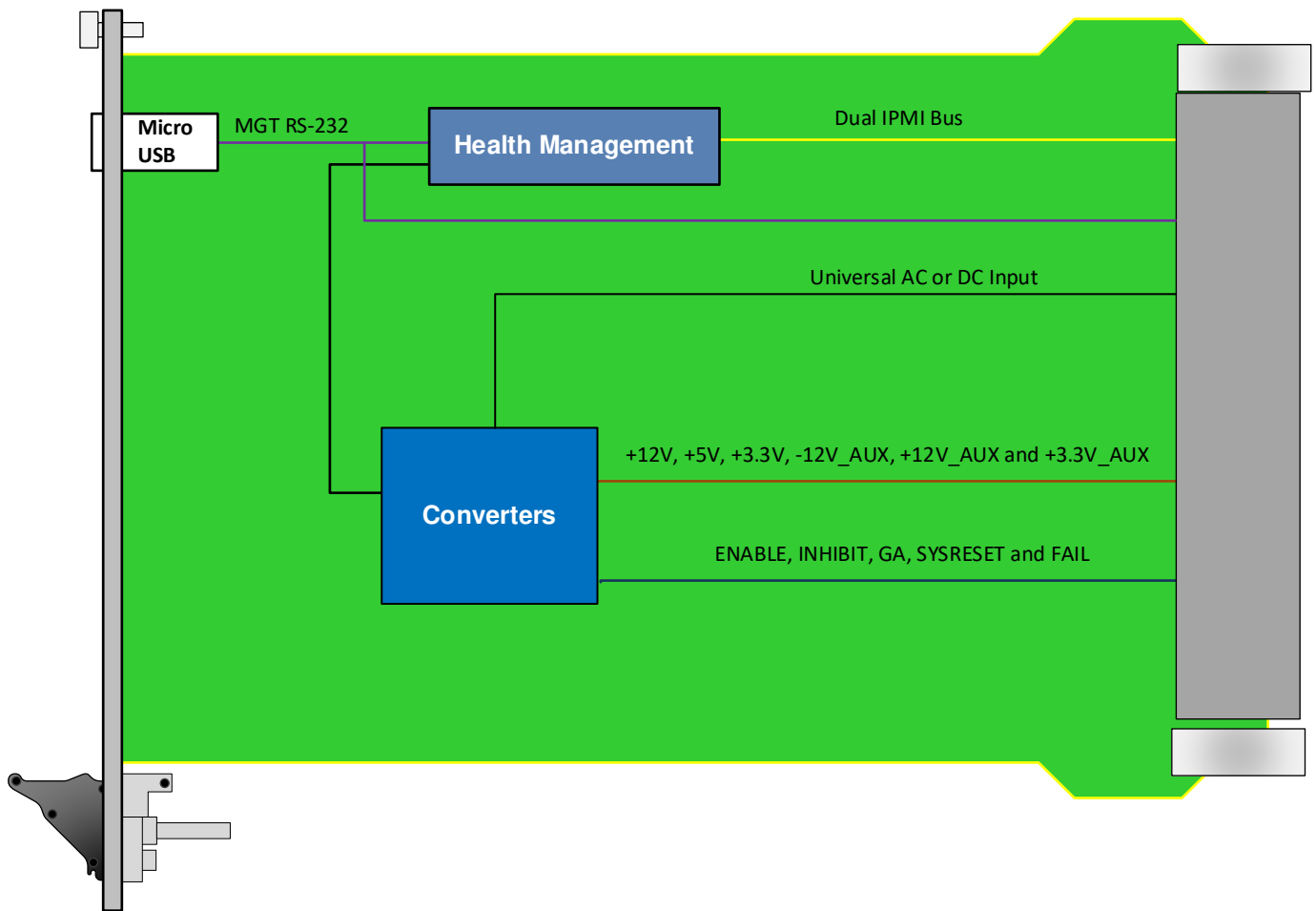
Figure 4: VPX020 Functional Block Diagram
