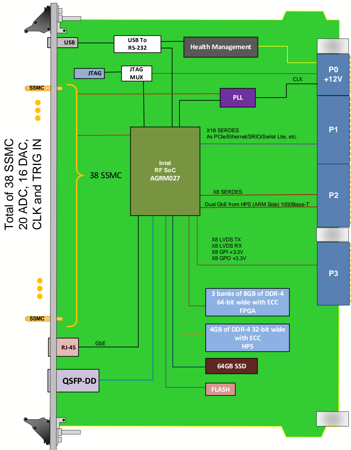
Figure 2: VPX540 Functional Block Diagram
