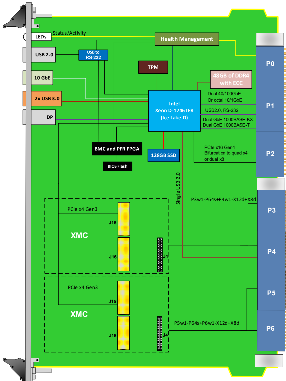
Figure 4: VPX775 Functional Block Diagram
