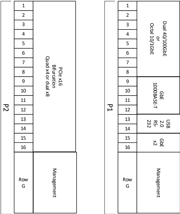
Figure 5: VPX775 Pinout Block Diagram
