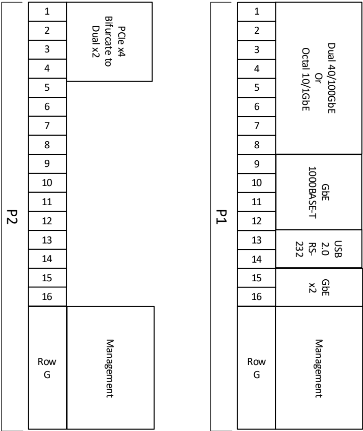
Figure 5: VPX779 Pinout Block Diagram
