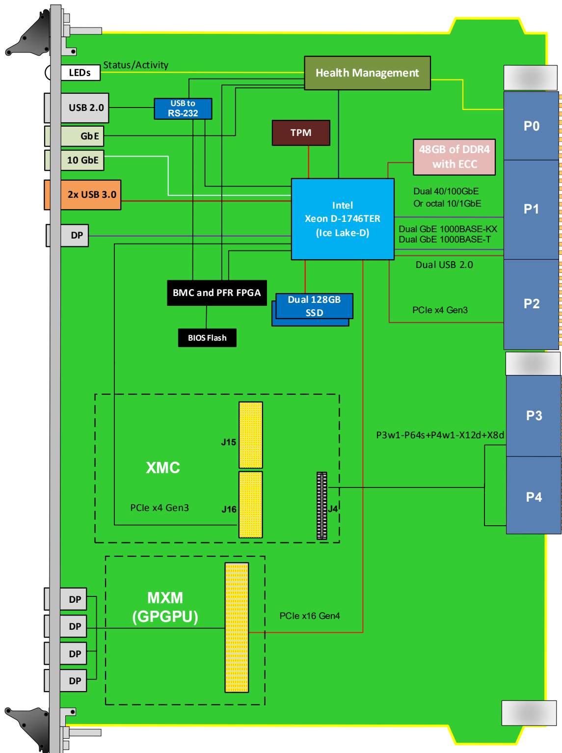
Figure 4: VPX779 Functional Block Diagram
