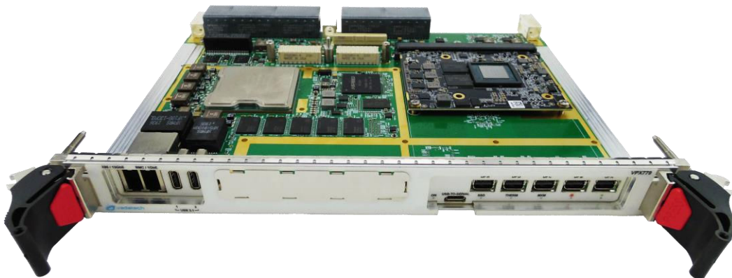
Figure 3: VPX779 Front View
