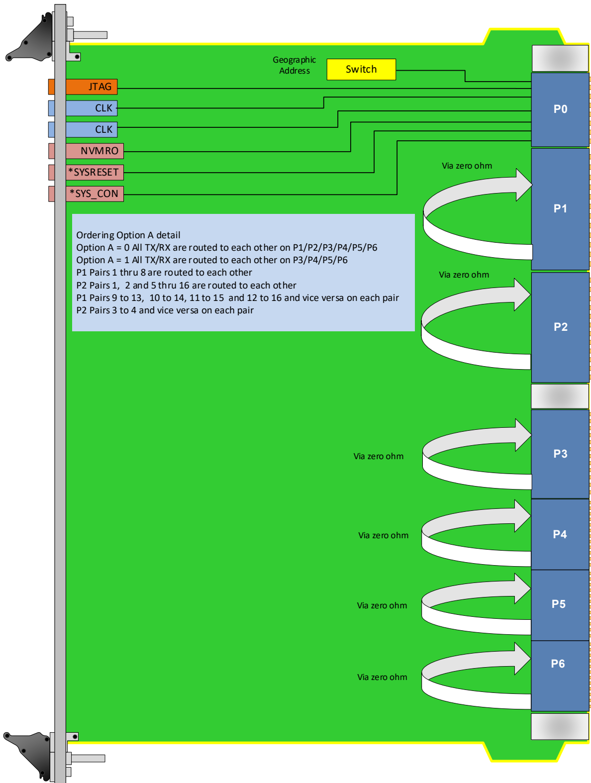
Figure 4: VPX998B Functional Block Diagram
