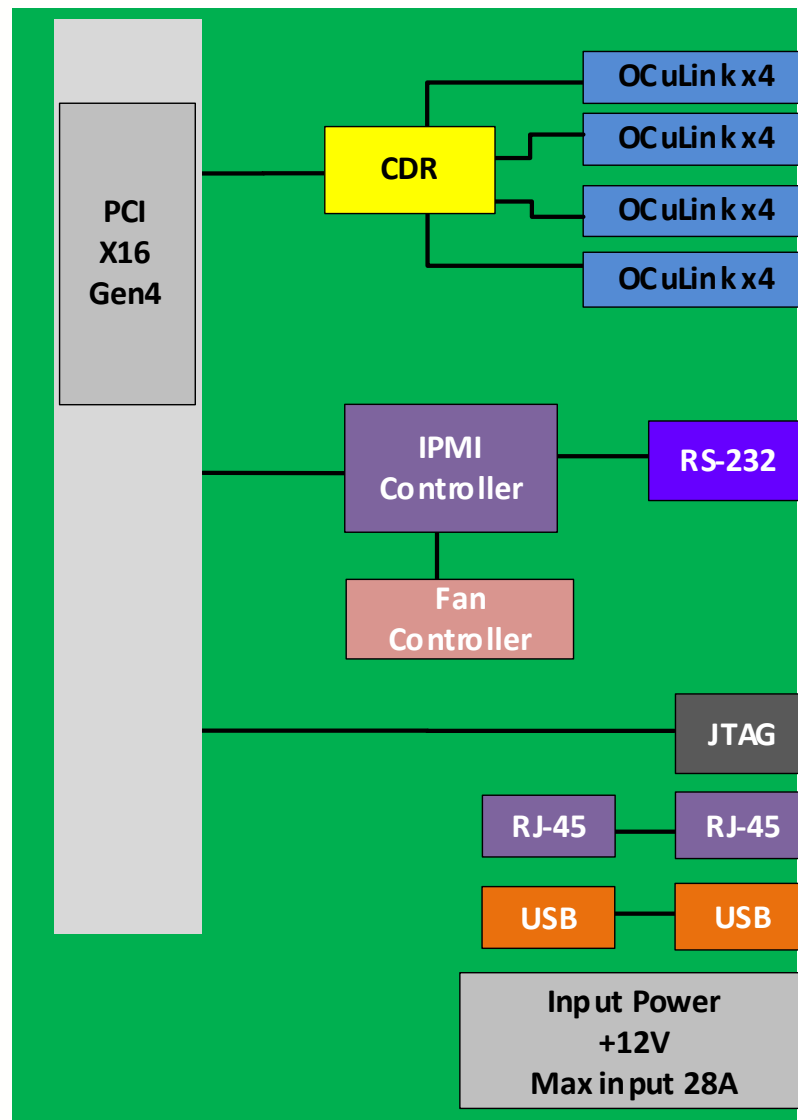
Figure 3: VT752 Module
