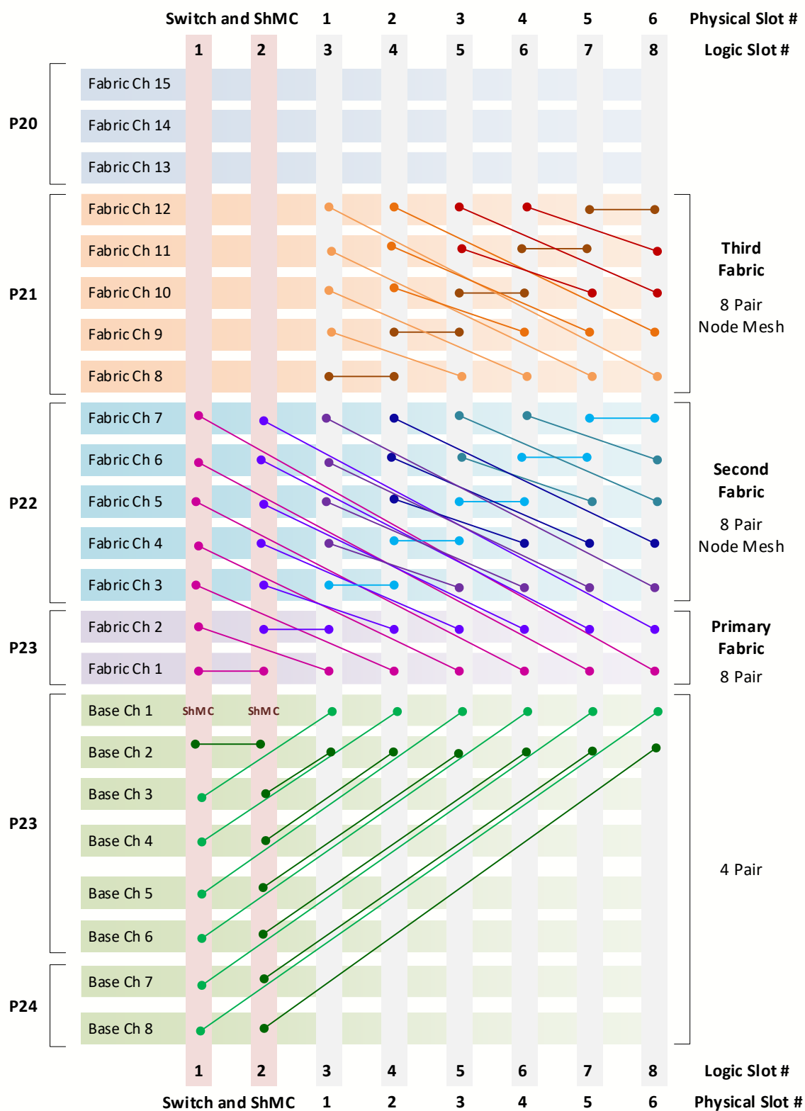
Figure 3: VT831 Backplane Full Mesh with a Replicated Mesh on Node slots
