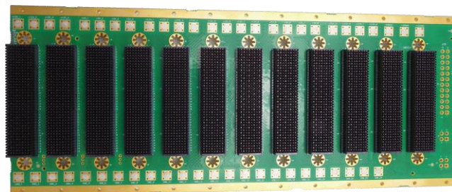
Figure 2: VTX353 Rear View
