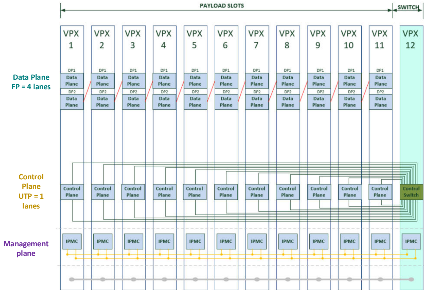
Figure 3: VTX353 Backplane Connections
