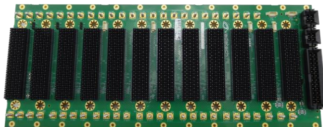
Figure 1: VTX353 Front View
